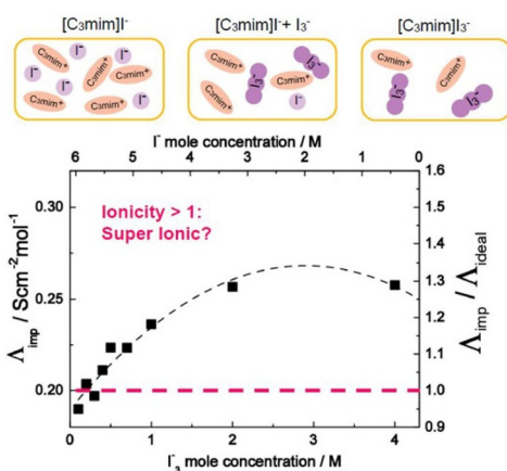
Fig. 5 Molar conductivity ( \Lambda_{imp} ) and ionicity ( \Lambda_{imp}/\Lambda_{ideal} ) of [C_3mim]I^- with added I_3^- as a function of I_3^- ( I^- ) concentration at iso-viscosity state of 0.2 Pa s. Reproduced from ref. 65 with permission from RSC, Copyright [2018].
