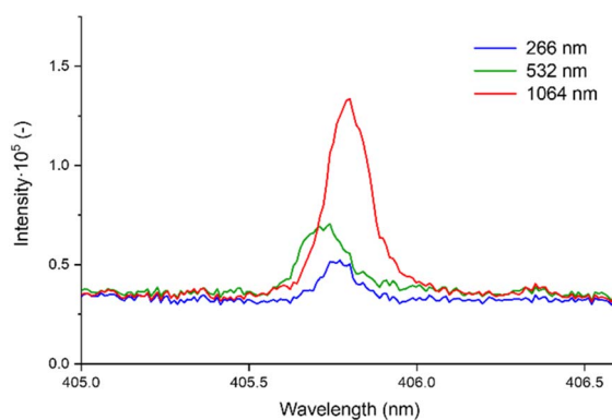
Fig. 4 Comparative analysis of signal intensities for Pb I 405.78 nm detection from all laser wavelengths acquired with optimal parameters from Table 5.
