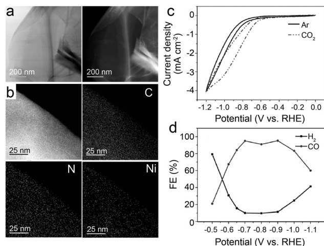
Fig. 2 (a) Representative TEM image of Ni-N-Gr (left) and corresponding high-angle annular dark-field scanning image (right). (b) High-resolution TEM image of Ni-N-Gr and corresponding EDX maps of C, N, and Ni. (c) Cyclic voltammograms of Ni-N-Gr catalyst in CO 2 -saturated 0.1 M KHCO 3 and Ar-saturated 0.1 M KH 2 PO 4 /K 2 HPO 4 (pH = 6.8) at 10 mV s -1 . (d) FEs for the reduction products generated by Ni-N-Gr catalyst. 35 Reprinted with permission from Wiley-VCH, copyright 2016.
