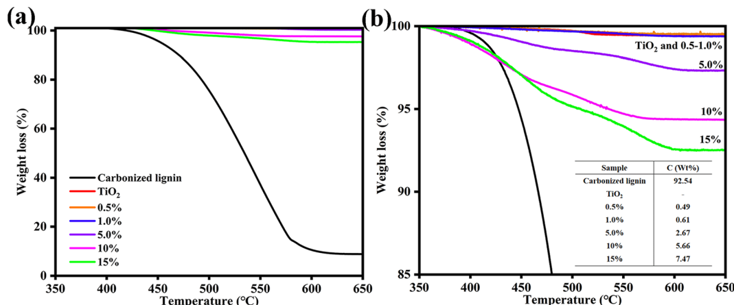
Fig. 3 (a) Tg and (b) the calculated C_{\text{lignin}} content of C_{\text{lignin}}@H\text{-TiO}_2 synthesized with different lignin weight percentages.
