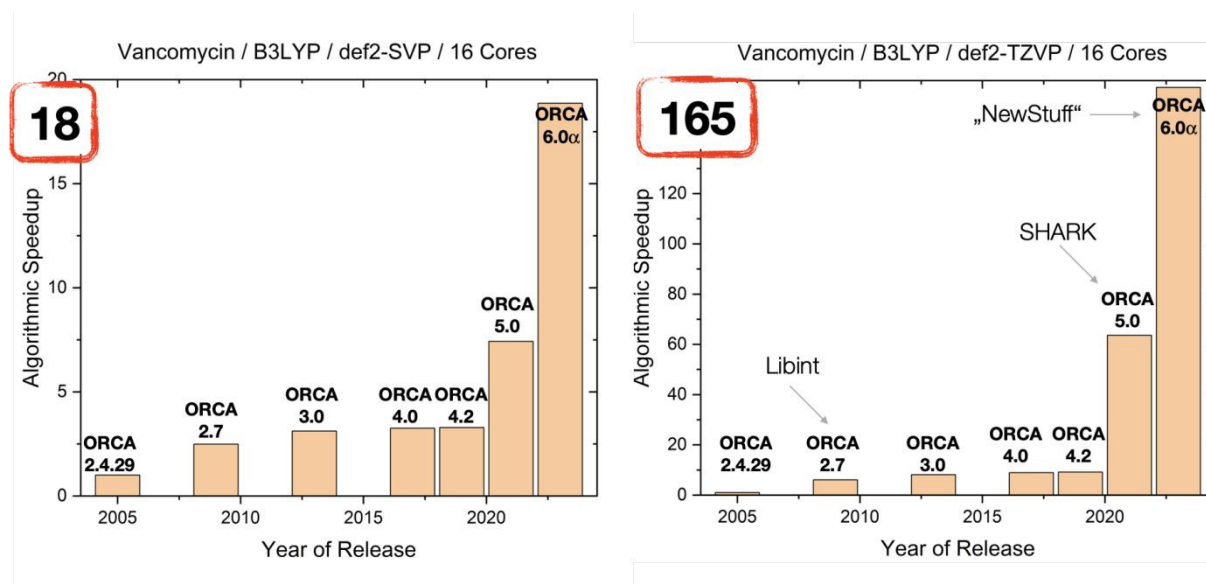
Figure 1: Algorithmic speedup over time relative to the early ORCA versions of 2005. The respective versions were all compiled with the same compiler, linked against the same libraries and run on the same computer. The test molecule was Vancomycin with 176 atoms. Left: def2-SVP basis set, right: def2-TZVP basis set.
