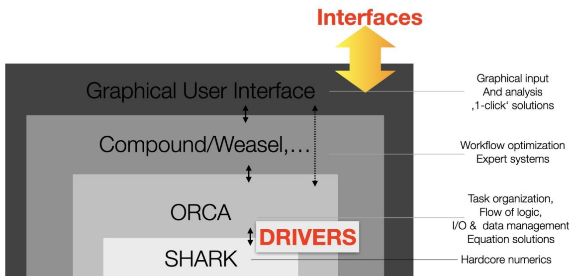
Figure 2: Illustration of the shell structure of the redesigned ORCA program package.
