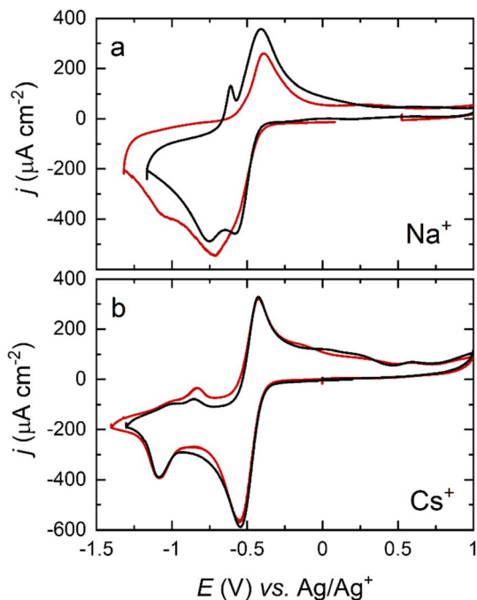
Fig. 6 Cyclic voltammograms of a Pt(111) (black) and a Pt(100) (red) electrode in an O 2 -saturated DMSO solution containing (a) 0.1 M NaClO 4 and (b) 0.1 M CsClO 4 . Scan rate: 50 mV s -1 .
