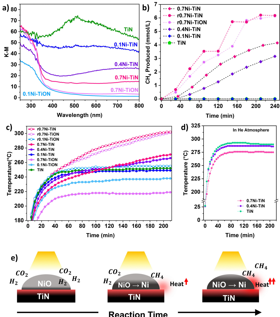
Fig. 2 (a) UV-vis absorption spectra for neat TiN, 0.1Ni-TiN, 0.4Ni-TiN, 0.7Ni-TiN and oxidised controls (0.1Ni-TiON, 0.7Ni-TiON); (b) photothermal \text{CH}_4 production by the various samples; (c) corresponding temperature profiles under photothermal conditions (Xe lamp at 20A setting); (d) xNi-TiN temperature profiles under inert He atmosphere ( \sim 80 kPa); (e) proposed photothermally-driven in situ Ni reduction mechanism.
