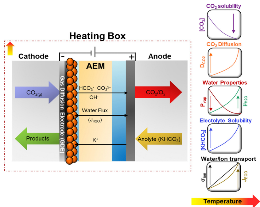
Fig. 1 Schematic representation of temperature dependency on transport and kinetics properties on \text{CO}_2\text{E} in zero-gap configuration. Equations for the presented trends for the different properties can be found in the ESI.†
