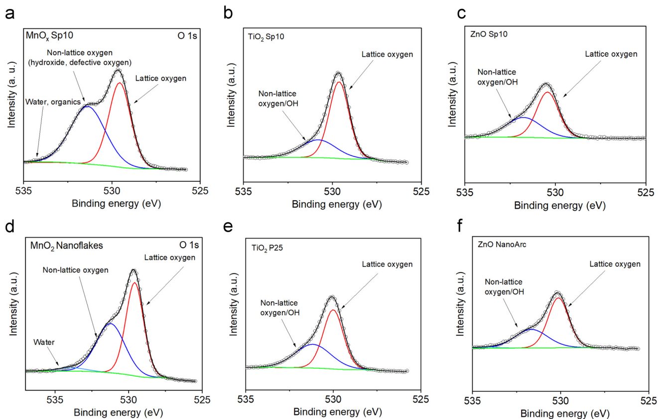
Fig. 11 High-resolution O 1s XPS spectra of spark-ablated a) manganese oxide ( \text{MnO}_x ), b) titanium dioxide ( \text{TiO}_2 ), and c) zinc oxide (ZnO) nanoparticles, respectively, and the comparison with O 1s XPS spectra of d) sol-gel prepared \text{MnO}_2 and commercial e) \text{TiO}_2 P25 and f) ZnO NanoArc. Peak deconvolution indicates the presence of lattice oxygen, non-lattice oxygen and/or adsorbed OH groups, and adsorbed water.
