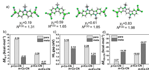
Fig. 4 (a) Isocontour plot of the FOD density ( \sigma = 0.005 \text{ e bohr}^{-3} ) and predicted N^{\text{FOD}} values together with the diradical character y_0 values of four DCM-substituted diradicals ( p -Cz-CN, 10,14 m -Cz-CN, 7,14 p -ICz-CN 15 and m -ICz-CN). (b) Comparison of the singlet–triplet gap (ΔE S-T ), (c) the HL gap and (d) the energy difference between OS and CS states (ΔE OS-CS ) of p -Cz-CN, 10,14 m -Cz-CN, 7,14 p -ICz-CN 15 and m -ICz-CN compounds at (U)M06-2X/6-31G** level of theory.
