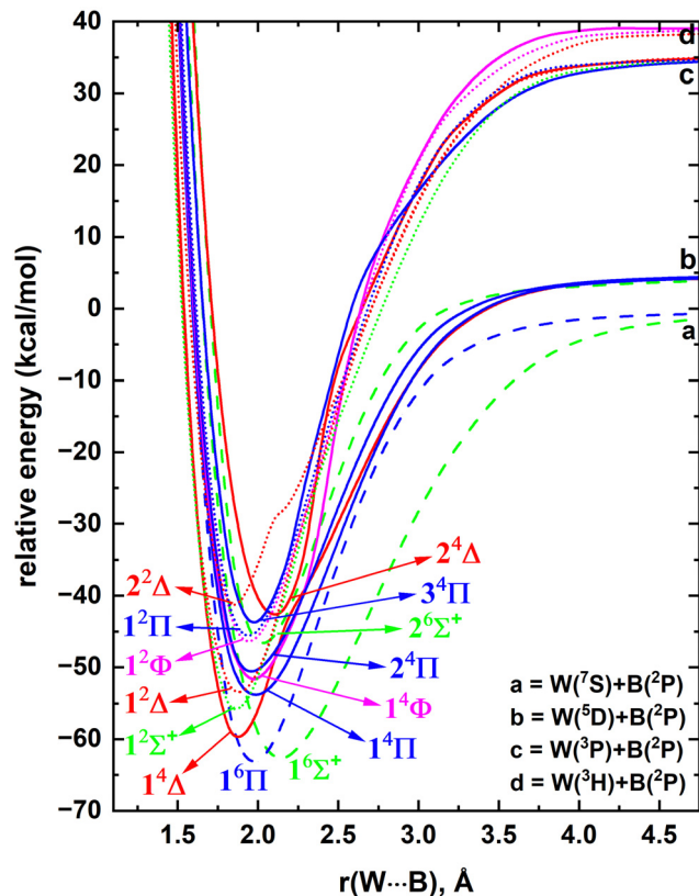
Fig. 6 Full MRCI PECs of WB as a function of W...B distance [r(W...B), Å]. The relative energies are referenced to the total energy of the W( 7 S) + B( 2 P) fragments at r = 200 Å, which is set to 0 kcal mol -1 . The Σ + , Π, Δ, and Φ states are shown in green, blue, red, and pink, respectively. The solid, dotted, and dashed PECs represent quartet, doublet, and sextet spins, respectively.
