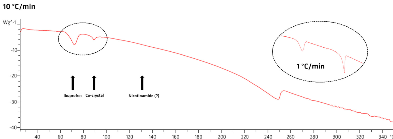
Fig. 6 10\text{ °C min}^{-1} DSC trace for the physical mixture ibuprofen–nicotinamide. It is evidenced the melting point of ibuprofen ( 78\text{ °C} ), of the co-crystal ( 90\text{ °C} ) and the one – missing – of nicotinamide ( 130\text{ °C} ). In the black dashed circle on the right, the 1\text{ °C min}^{-1} DSC of the physical mixture to better appreciate the formation of the co-crystal among melting.
