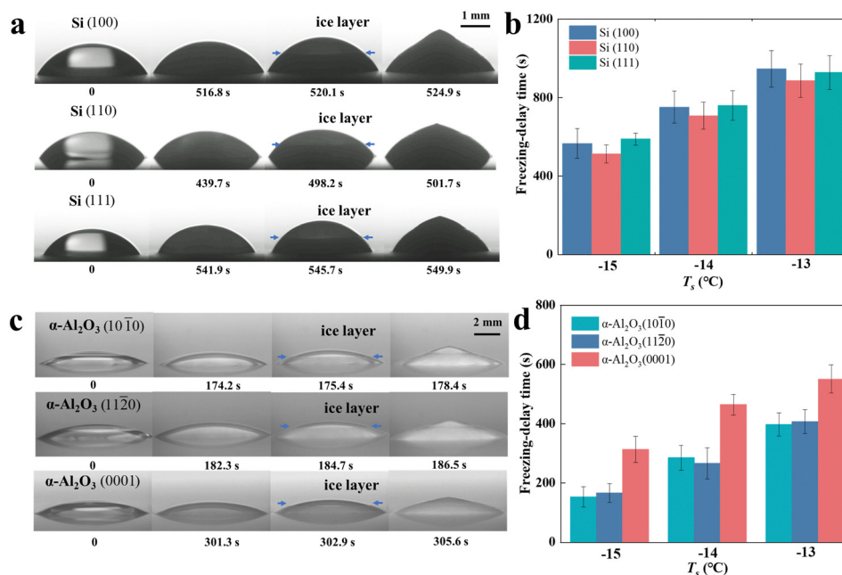
Fig. 2 (a) A droplet with a volume of 10 \mu\text{L} freezes on a silicon substrate at T_s = -15 ^{\circ}\text{C} . (b) The freezing delay time of the droplet on silicon substrates. (c) A droplet with a volume of 10 \mu\text{L} freezes on \alpha\text{-Al}_2\text{O}_3 substrates at T_s = -15 ^{\circ}\text{C} . (d) The freezing delay time of the droplet on \alpha\text{-Al}_2\text{O}_3 substrates. The smaller the \delta_d , the shorter the freezing delay time. The \delta_d values for Si (100), \alpha\text{-Al}_2\text{O}_3 (10 \bar{1}0 ) and \alpha\text{-Al}_2\text{O}_3 (11 \bar{2}0 ) are 1.9%, 5.2% and 5.2%, which are smaller than other crystal planes. Thus, freezing occurs easily on these substrates above. The error bar is the error of the mean.
