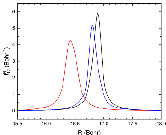
Fig. 6 Non-adiabatic coupling elements r_{12}^{12} between the lowest two LiCN states of ^1A' symmetry at fixed \theta = 90^\circ and r = 2.1 bohr (red), 2.22 bohr (black) and 2.35 bohr (blue).
