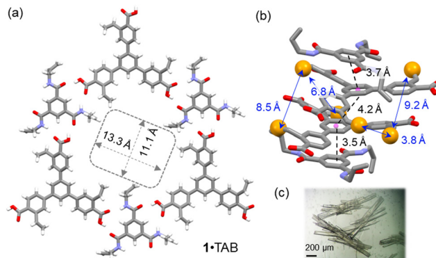
Fig. 1 (a) Single-crystal structure of the 1·TAB co-crystal viewed along the b/c plane. (b) The ABBA-type alternative packing of 1 and TAB, viewed along the a -axis. The \pi - \pi stacking distances and distances between the terminal carbon atoms of the styrene moieties are highlighted. (c) An image of 1·TAB co-crystals.
