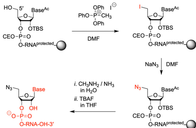
Fig. 4 Solid-phase synthesis of 5'-azido modified oligoribonucleotides. Reagents and conditions: (1) 0.5 M MTPI/DMF, rt, 1 h; (2) sat. NaH 2 PO 4 solution in DMF, 55 °C, 5 h; (3) (i) 40% aq MeNH 2 /30% aq NH 3 (1/1 v/v), 40 °C, 4 h, (ii) 1 M TBAF/THF, 37 °C, 16 h.
