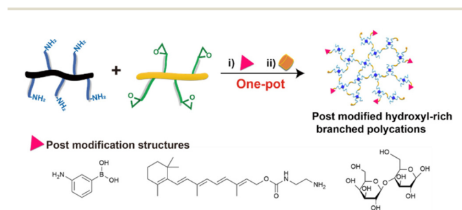
Fig. 5 One-pot poly-amine and poly-epoxy ring-opening reaction for the construction of post modified branched hydroxyl-rich polycations.
