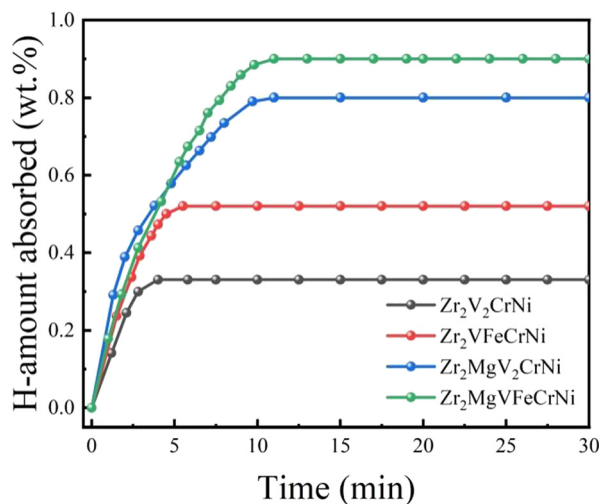
Fig. 5 Hydrogen absorption kinetics curves of \text{Zr}_2\text{Mg}_x\text{V}_{2-y}\text{Fe}_y\text{CrNi} ( x = 0 and 1 , and y = 0 and 1 ) high-entropy alloys at 303\text{ K} .
