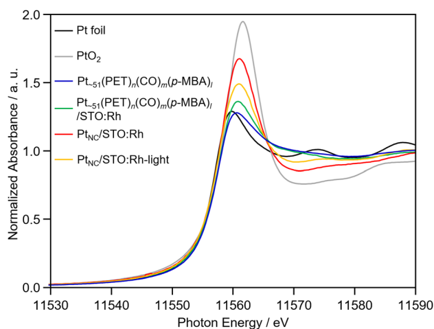
Fig. 4 Pt L_3 -edge XANES spectra of \text{Pt}_{\sim 51}(\text{PET})_n(\text{CO})_m(\textit{p}\text{-MBA})_l , before ( \text{Pt}_{\sim 51}(\text{PET})_n(\text{CO})_m(\textit{p}\text{-MBA})_l/\text{STO:Rh} ) and after ( \text{Pt}_{\text{NC}}/\text{STO:Rh} ) calcination of Pt NC-loaded STO:Rh, and after light irradiation onto \text{Pt}_{\text{NC}}/\text{STO:Rh} ( \text{Pt}_{\text{NC}}/\text{STO:Rh-light} ). Pt foil ( \text{Pt}^0 ) and \text{PtO}_2 powder ( \text{Pt}^{4+} ) were also shown for comparison. A stronger and weaker absorbance indicates a more oxidized and reduced electronic state of Pt at the whiteline, respectively.
