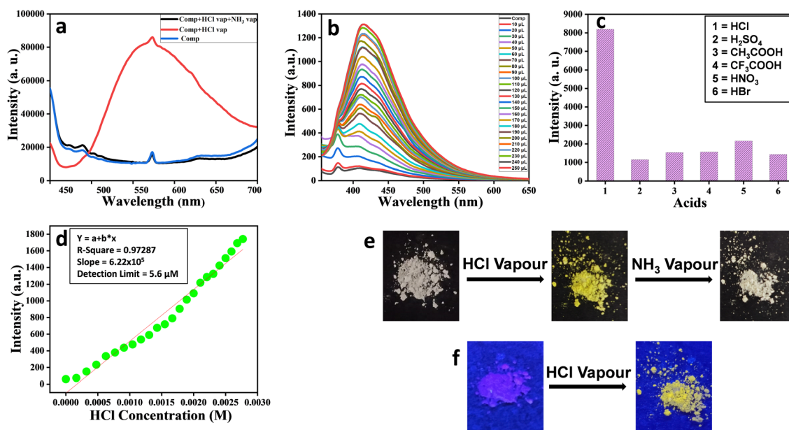
Fig. 8 (a) Fluorescence spectra of mesogen P-11 in the solid state when exposed to HCl vapour and NH 3 vapour (338 nm). (b) Fluorescence spectra of P-11 (10 -5 M in THF) recorded before and after its exposure to different concentrations of HCl solution (10 -2 M in acetonitrile). (c) Fluorescence intensity of compound P-11 after the addition of 50 μL of 10 -2 M solution of various acids to the stock solution. (d) Calibration curve of the fluorescence intensity versus HCl concentration. Optical photographs of P-11 upon exposure to HCl vapour and ammonia vapour under normal light (e), and upon exposure to HCl vapour under UV light (f).
