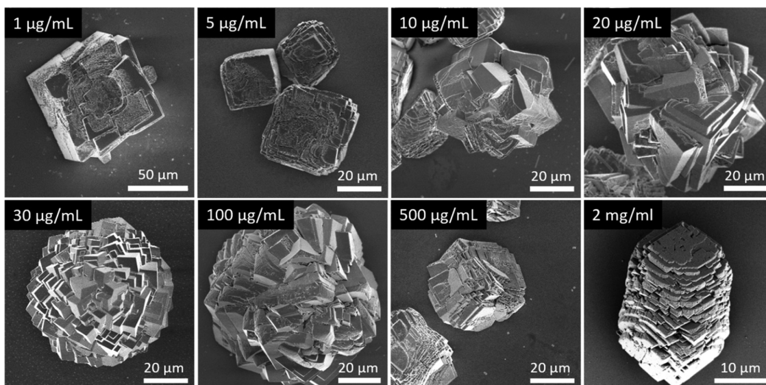
Fig. 5 Effect of peptide A-04-17 on the in vitro mineralization of CaCO 3 . The aragonite-binding peptide was applied in the bioinspired mineralization of CaCO 3 via a slow diffusion of NH 3 and CO 2 induced by the decomposition of ammonium carbonate into a CaCl 2 solution. The mineralization was performed in the presence of protein concentrations ranging from 1 μg mL -1 to 2 mg mL -1 .
