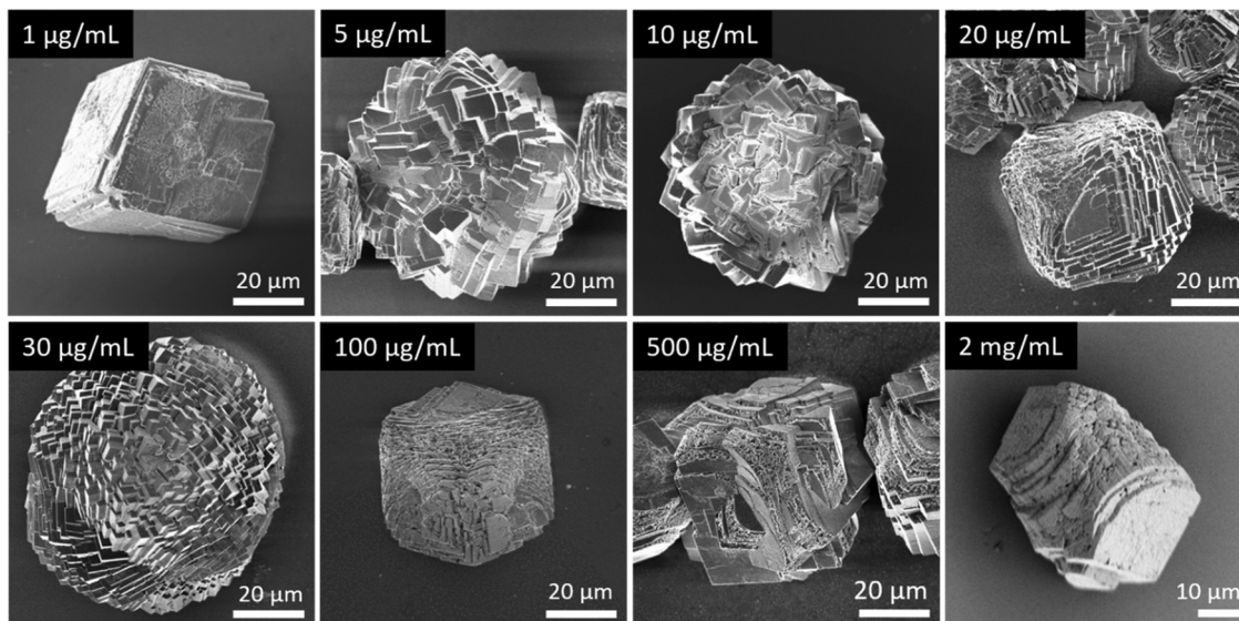
Fig. 4 Effect of peptide A-04-09 on the in vitro mineralization of CaCO 3 . The aragonite-binding peptide was applied in the bioinspired mineralization of CaCO 3 via a slow diffusion of NH 3 and CO 2 induced by the decomposition of ammonium carbonate into a CaCl 2 solution. The mineralization was performed in the presence of protein concentrations ranging from 1 μg mL -1 to 2 mg mL -1 .
