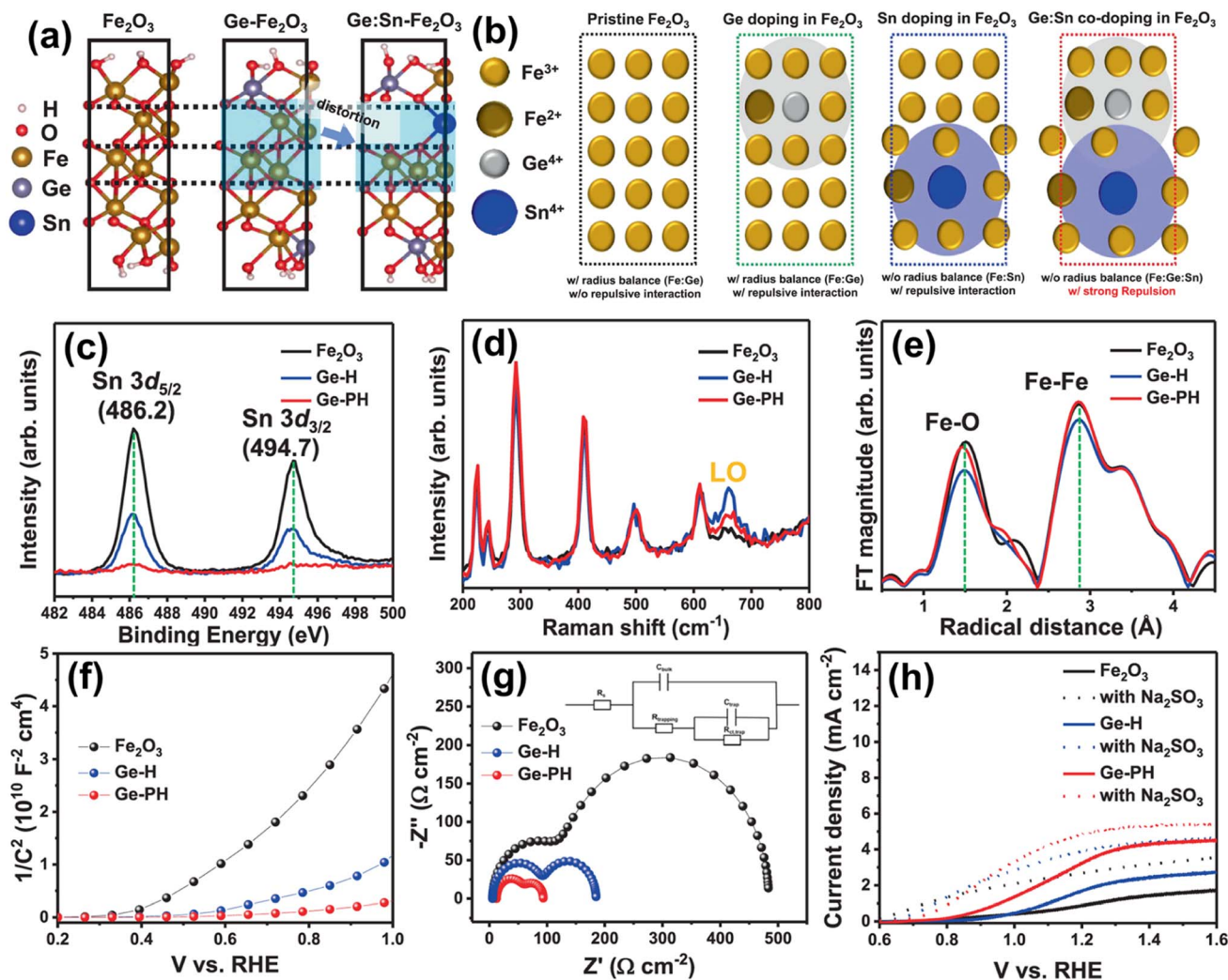
Fig. 13 (a) DFT calculations of atomic arrangements of Fe 2 O 3 with different dopant environments. (b) Atomic structure of Ge-doped Fe 2 O 3 , Sn-doped Fe 2 O 3 and Ge:Sn co-doped Fe 2 O 3 . (c) XPS spectra of Sn. (d) Raman spectra. (e) Fourier transform of the EXAFS data at the Fe k-edge of the hematite nanostructures. (f) Mott-Schottky plots and (g) EIS measurements (with the circuit model). (h) J - V curves of Fe 2 O 3 , Ge-H, and Ge-PH under illumination in 1 M NaOH (solid line) and a solution mixture of 1 M NaOH and 0.5 M Na 2 SO 3 (dashed lines). Reproduced from ref. 67 with permission from Springer Nature, Copyright 2021.
