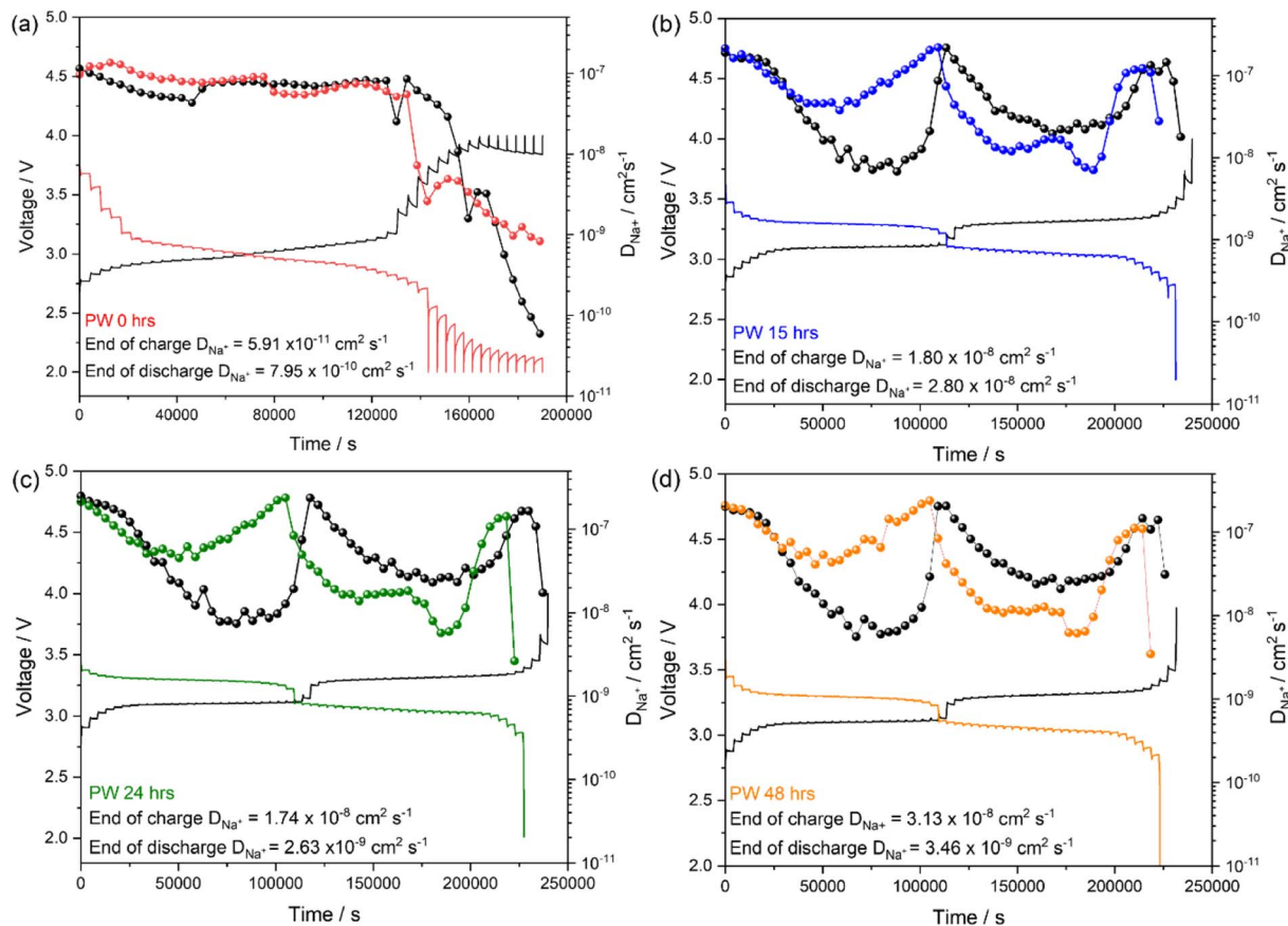
Fig. 10 GITT curves and corresponding calculated D_{Na^+} upon sodiation/de-sodiation for (a) undried (b) 15 hours, (c) 24 hours and (d) 48 hours PW electrodes dried at 170 °C under a dynamic vacuum of 10^{-3} mbar.
