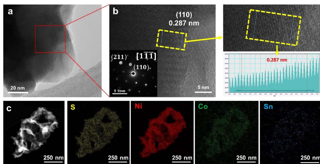
Fig. 3 Physicochemical analysis of catalysts. (a) HRTEM image and (b) enlarged image with SAED pattern of CoSn-Ni 3 S 2 @NF. The right inset shows an atomic resolution image of yellow dashed box. (c) EDX spectra of each element of CoSn-Ni 3 S 2 @NF. (d) Nitrogen adsorption-desorption isotherms and (e) total pore volume and pore size of Ni 3 S 2 @NF, Co-Ni 3 S 2 @NF, and CoSn-Ni 3 S 2 @NF.
