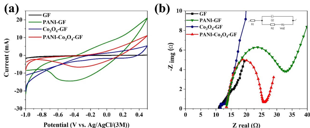
Fig. 4 Electrochemical characterisation of the anode electrodes before use. (a) CV scans at 0.01 \text{V s}^{-1} and (b) EIS spectra. Tests were performed in a 3-electrode system in 50 mM PBS (pH 7), with the anode as the working electrode and Pt wire (diameter: 0.127 mm) as the counter electrode.
