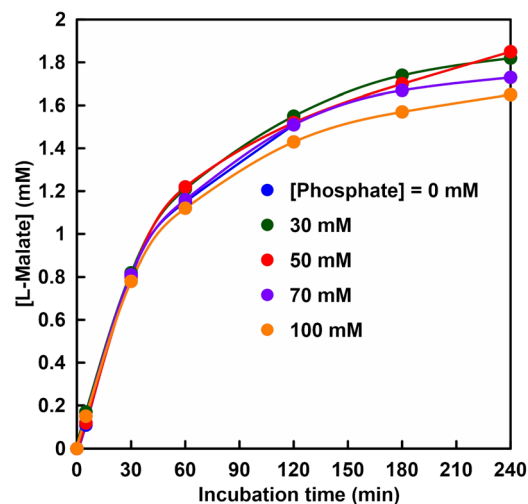
Fig. 8 Time course of L-malate production with the system of sodium pyruvate, NADH, magnesium chloride, sodium bicarbonate and ME in CO 2 saturated HEPES buffer containing various phosphate concentrations.
