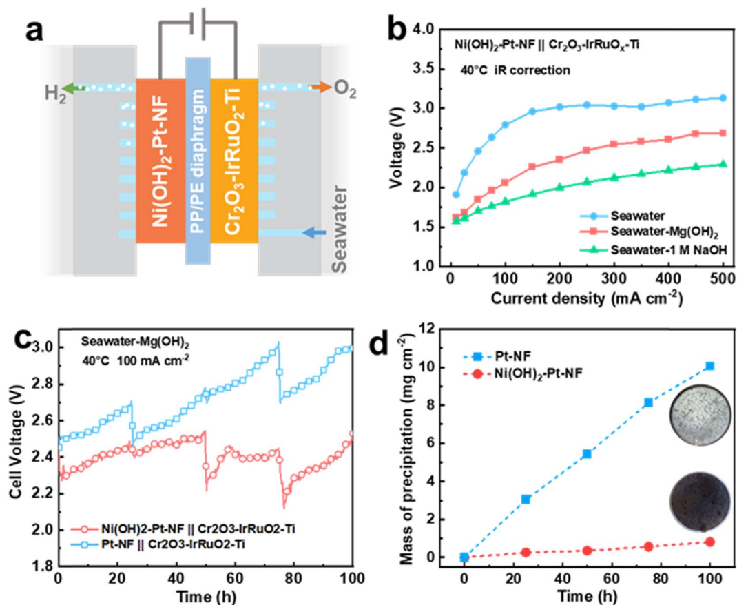
Fig. 6 (a) A schematic illustration of a direct seawater electrolyser equipped with an \text{Ni}(\text{OH})_2 -Pt-NF electrode. (b) The polarization curves of an \text{Ni}(\text{OH})_2 -Pt-NF-electrode-equipped electrolyser in different electrolytes. (c) Galvanostatic discharge curves of electrolyzers at a current density of 100 \text{ mA cm}^{-2} and (d) mass of precipitation on the \text{Ni}(\text{OH})_2 -Pt-NF and Pt-NF electrodes (inset: photographs of the HER electrodes after 100 h of measurement).
