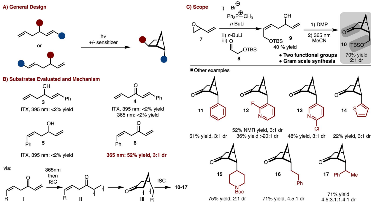
Scheme 1 Crossed [2 + 2]-cycloaddition.
