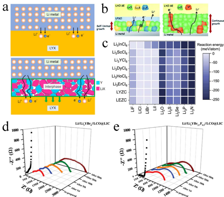
Fig. 17 (a) Schematic illustration of the reaction of LYX electrolyte and the Li anode. Once LYX electrolyte was in contact with Li metal, it was reduced to form a Y and LiX interphase that could conduct both Li + and electrons, allowing the adverse side reaction to continue. Reproduced with permission. 152 Copyright 2021, Science China Press and Springer. (b) Schematic illustration showing the mechanism of LPSCl action on the interface stability. Reproduced with permission. 153 Copyright 2021, The Royal Society of Chemistry. (c) Heatmap of the reaction energy between binary coating materials and lithium chloride electrolyte. Reproduced with permission. 145 Copyright 2021, American Chemical Society. The EIS evolution at different cycles of (d) Li/Li 3 YBr 6 //LCO@LIC and (e) Li/Li 3 YBr 5.7 F 0.3 //LCO@LIC cells. Reproduced with permission. 146 Copyright 2021, Wiley-VCH.
