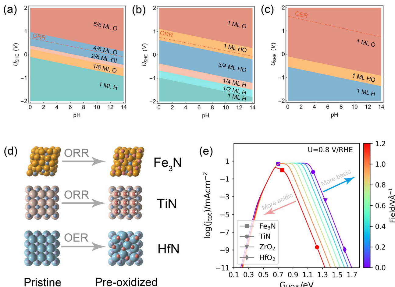
Fig. 6 Calculated 2D surface Pourbaix diagrams as a function of potential (vs. SHE) and pH ( T = 298.15 \text{ K} ) for (a) Fe 3 N(111), (b) TiN(100), and (c) HfN(100). (d) Corresponding atomic structures before and after surface state changes. Yellow, brown, cyan, blue, red, and white spheres denote Fe, Ti, Hf, N, O, and H atoms, respectively. (e) Derived pH-dependent volcano activity model for the ORR as a function of HO* adsorption (at 0.8 V vs. RHE) plotted with the Fe 3 N(111), TiN(100), ZrO 2 (111), and HfO 2 (111) under their identified surface states under ORR conditions. Note: the pristine surfaces were previously identified to be favorable under ORR conditions for ZrO 2 and HfO 2 (111). 19
