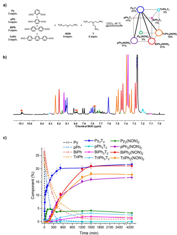
Fig. 10 (a) [4 \times 2] square prismatic DC ov L generated from 3Py + 3pPh + 3BiPh + 3TriPh + 2T + 9NON; (b) partial ^1\text{H} NMR spectrum (400 MHz, \text{CDCl}_3 , 40 °C) of the equilibrated reaction mixture; (c) ^1\text{H} NMR monitoring of macrocycles and macrocyclic cages over 4260 min. The initial concentration of each dialdehyde was 2.0 mM. The signals of free dialdehydes BiPh and TriPh are indicated by red and orange stars, respectively. The larger size and the bold diagonal lines indicate the selective cogeneration of agonistic constituents. The spectra and kinetic curves are coloured in accordance with the molecular structures.
