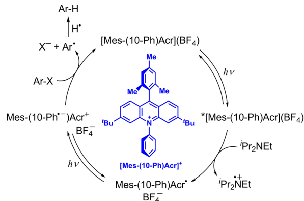
Scheme 4 Reductive dehalogenation of aryl halide ( \text{Ar-X} ) with diisopropylamine by photoredox catalysis of [\text{Mes}-(10\text{-Ph})\text{Acr}](\text{BF}_4) . 37
