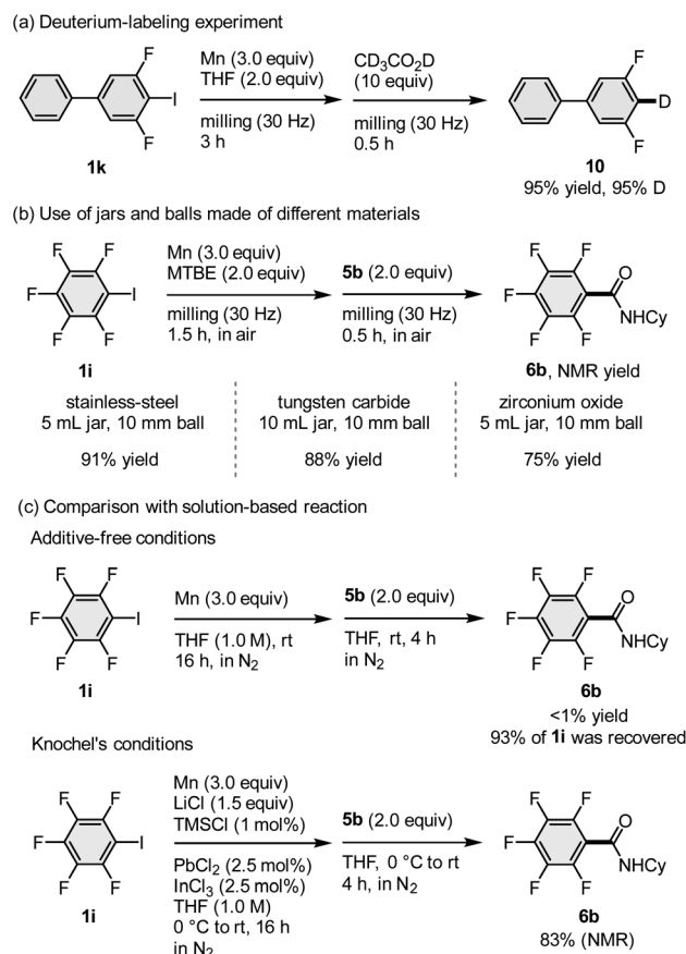
Scheme 4 Mechanistic studies. (a) Deuterium-labeling study. (b) Effect of milling jars and balls made of different materials. (c) Comparison with solution-based conditions. ^{\ddagger} For the reaction conditions, please see the ESI.†
