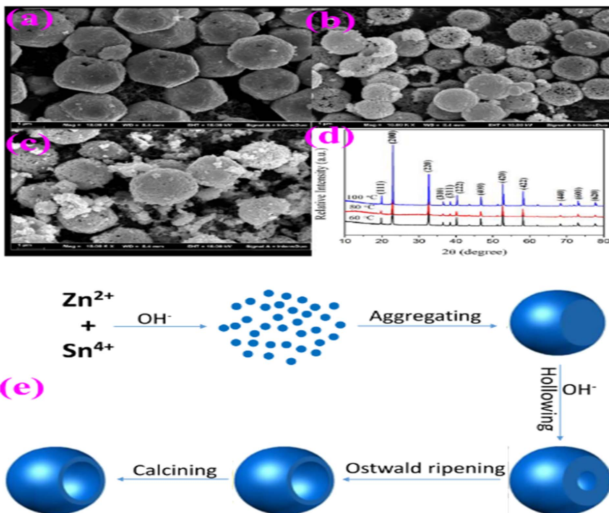
Fig. 14 SEM images of \text{ZnSnO}_3 obtained at different reaction temperatures: (a) 60 ^\circ\text{C} , (b) 80 ^\circ\text{C} , and (c) 100 ^\circ\text{C} . (d) XRD patterns of \text{ZnSn(OH)}_6 precursor. (e) Schematic illustration of the possible formation mechanism of \text{ZnSnO}_3 hollow spheres. 70
