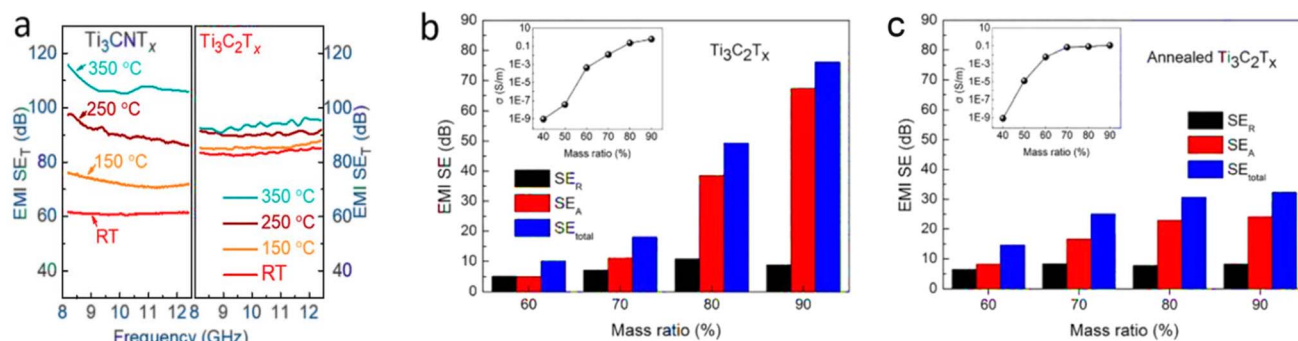
Fig. 20 (a) comparison between \text{Ti}_3\text{CNT}_x and \text{Ti}_3\text{C}_2\text{T}_x with regard to annealing temperature. (b and c) Annealing effect for \text{Ti}_3\text{C}_2\text{T}_x /wax composites. Reproduced from ref. 340 with permission from American Chemical Society, copyright 2016.
