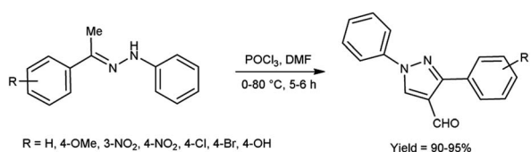
Scheme 22 Synthesis of 1-phenyl-3-substitutedphenyl-1H-pyrazole-4-carbaldehydes.
