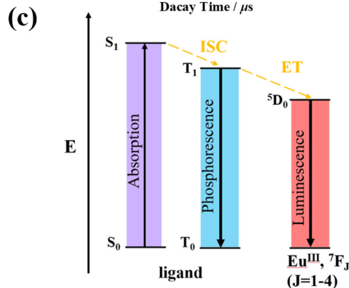
Fig. 5 (a) Excitation and emission spectra; (b) luminescence lifetime; and (c) Jablonsky level diagrams of \text{Eu}_{28} .
