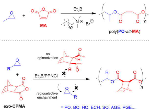
Scheme 11 Selective copolymerization of epoxides and anhydrides (including tricyclic ones) using Et 3 B-cocatalysis.
