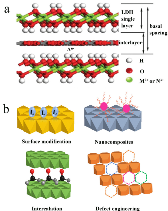
Fig. 1 (a) Schematic of the LDH structure. Reprinted with permission from ref. 30. Copyright 2020, Royal Society of Chemistry. (b) Schematic illustration of four ways of LDH functionalization.
