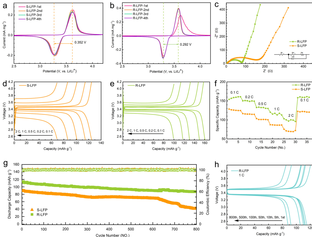
Fig. 4 Electrochemical performances of S-LFP and R-LFP. CV curves of (a) S-LFP and (b) R-LFP; (c) Nyquist plots of R-LFP and S-LFP; charge-discharge curves of (d) S-LFP and (e) R-LFP at different rates; (f) rate performance of samples; (g) long-term cycling stability of S-LFP and R-LFP; (h) charge-discharge curves of R-LFP after several cycles.
