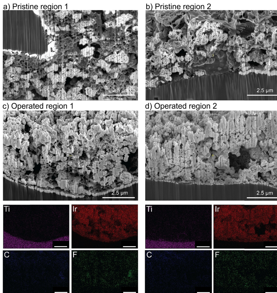
Fig. 9 Cross-sectional analysis of \text{IrO}_x /mixed binder anode PTE. SEM images of different regions of the pristine catalyst layer (a) and (b) and SEM with EDX maps of two operated regions (c) and (d). Only PTFE binder is observed in the catalyst layer after operation.
