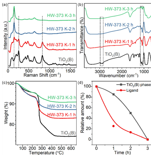
Fig. 3 (a) Raman and (b) FT-IR spectra and (c) TGA results of the \text{TiO}_2(\text{B}) nanosheets and samples obtained after heating in water at 373 K for 1, 2 and 3 hours; and (d) calculated mass ratio of the \text{TiO}_2(\text{B}) phase and residual EG ligand.
