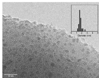
Fig. 18 (A) TEM image of 5 wt% Ni/MOR catalyst and (B) long-term partial oxidation of methane over the Ni/MOR catalyst. Reaction conditions: \text{CH}_4/\text{O}_2/\text{Ar} = 0.06/0.03/0.91 atm; \text{SV} = 3.0 \times 10^4 \text{ mL h}^{-1} \text{ g}_{\text{cat}}^{-1} ; 973 K. Reproduced from ref. 77 with permission from Springer Nature, copyright 2020.
