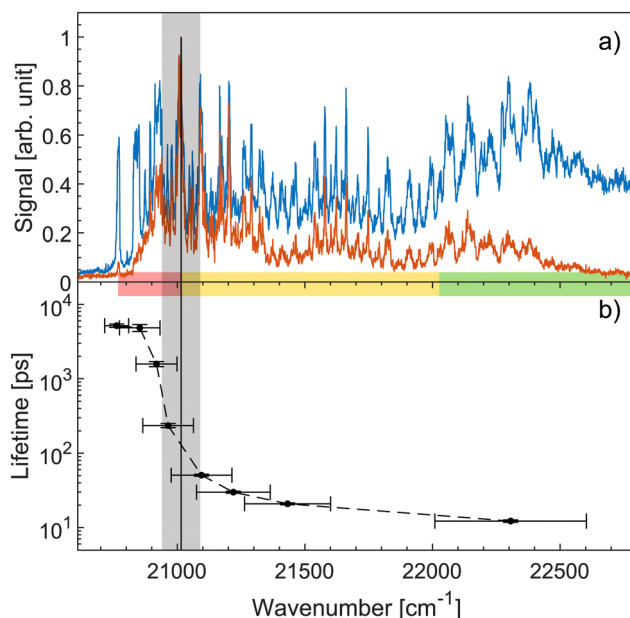
Fig. 4 (a) Action-absorption spectra of \text{HBDI}^- reported recently. 31 The blue curve is the prompt-detachment signal and the red curve is the signal corresponding to detection of mass 200 amu photo-fragmentation signal (loss of methyl). (b) The lifetime as a function of photon energy. The horizontal errorbars are the FWHM of the pump pulses, while the vertical errorbars are from the exponential fit to the data. The vertical black line is the energy barrier-top position proposed based on the spectroscopy 31 and the grey band indicates the energy-barrier top position estimated from the sudden change in lifetime. Notice the logarithmic scale showing over two orders of magnitude span in lifetimes. The energy-barrier height is determined as the difference between the band origin at 20\,768\text{ cm}^{-1} and the energy-barrier top position. The horizontal colored bar indicates the different spectral regions, also shown in Fig. 2 and 3.
