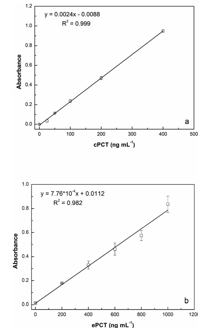
Fig. 5 Linear fitting obtained for cPCT on cMIPs and ePCT on eMIPs in species-specific plasma (diluted 1 : 10) with the sandwich assay (nonspecific signals were subtracted).
