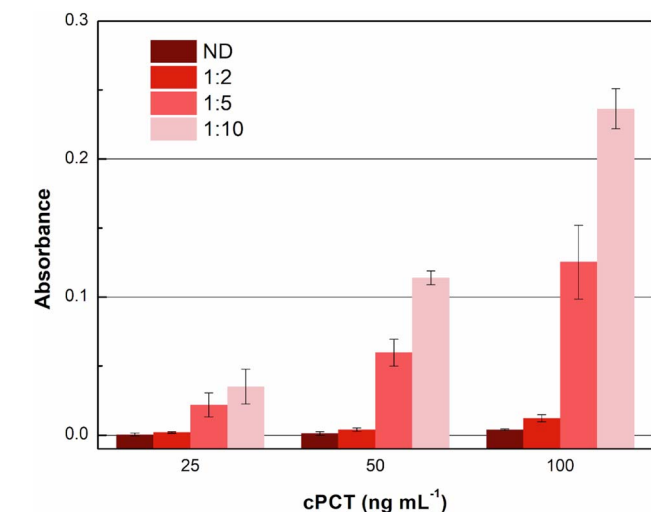
Fig. 4 Procalcitonin (PCT) sandwich assays in canine plasma samples diluted and fortified with cPCT (25.0, 50.0, 100 ng mL -1 ). Samples were tested undiluted (ND) and at different dilutions (1 : 2, 1 : 5 and 1 : 10, respectively). Three replicates for each concentration.
