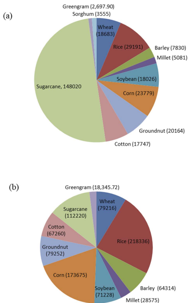
Fig. 5 (a) and (b): Global average variation in input and output energy ( \text{MJ ha}^{-1} ) of different crops.
