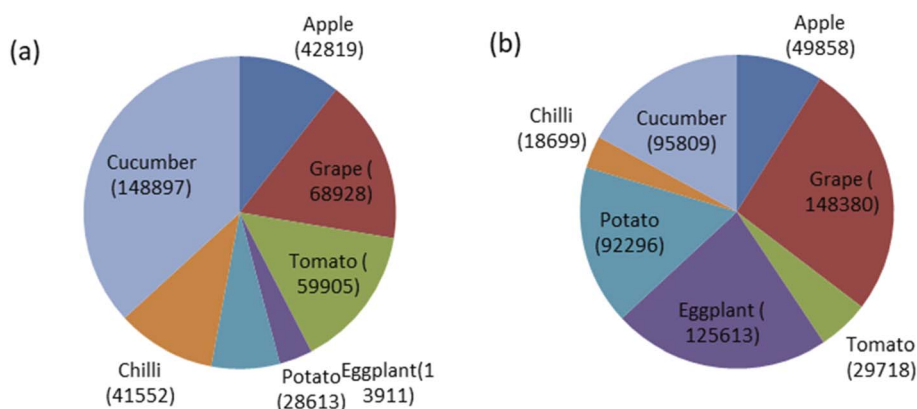
Fig. 6 (a) and (b) Global average variation in input and output energy ( \text{MJ ha}^{-1} ) of horticultural crops.
