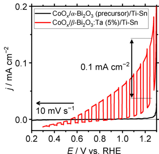
Fig. 10 LSV at 10 mV s -1 under light chops for CoO x /α-Bi 2 O 3 (precursor)/Ti-Sn and CoO x /β-Bi 2 O 3 :Ta (5%)/Ti-Sn in 1 M potassium borate aqueous solution (pH 9). Sacrificial reagent: 0.1 M Na 2 SO 3 ; RE: Hg/Hg 2 Cl 2 /saturated KCl; CE: Pt wire; light source: Xe-lamp (MAX-303, 300 W) with cut-off filter (L42), > 420 nm; temperature: 25 °C.
