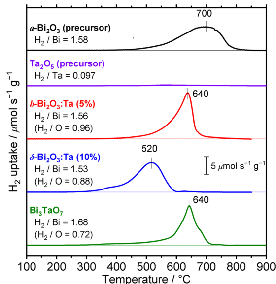
Fig. 11 TPR profiles of α-Bi 2 O 3 (precursor), Ta 2 O 5 (precursor), β-Bi 2 O 3 :Ta (5%), δ-Bi 2 O 3 :Ta (10%), and Bi 3 TaO 7 . The total hydrogen consumptions are expressed in moles of H 2 consumed per mole of metal atoms (H 2 /Bi or H 2 /Ta) and moles of H 2 consumed per mole of O atoms (H 2 /O). The samples were pretreated in Ar (20 mL min -1 ) at 400 °C before each measurement. The measurements were conducted on 20 mg of samples in 4% H 2 (in Ar, 20 mL min -1 ) with a heating rate of 10 °C min -1 .
