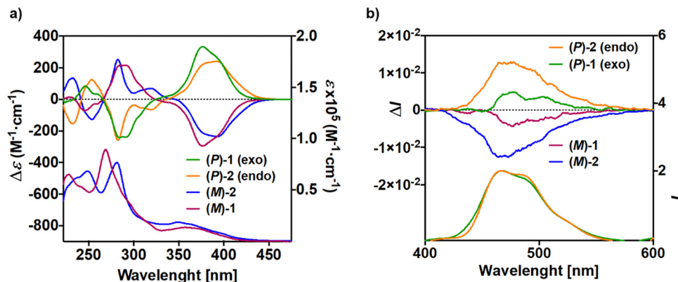
Fig. 2 (a) Experimental UV-vis (bottom) and ECD (top) spectra and (b) fluorescence (bottom) and CPL (top) spectra of ( P ) and ( M ) enantiomers of 1 and 2 ( \text{CH}_2\text{Cl}_2 , C \sim 10^{-5} \text{ M} ).
