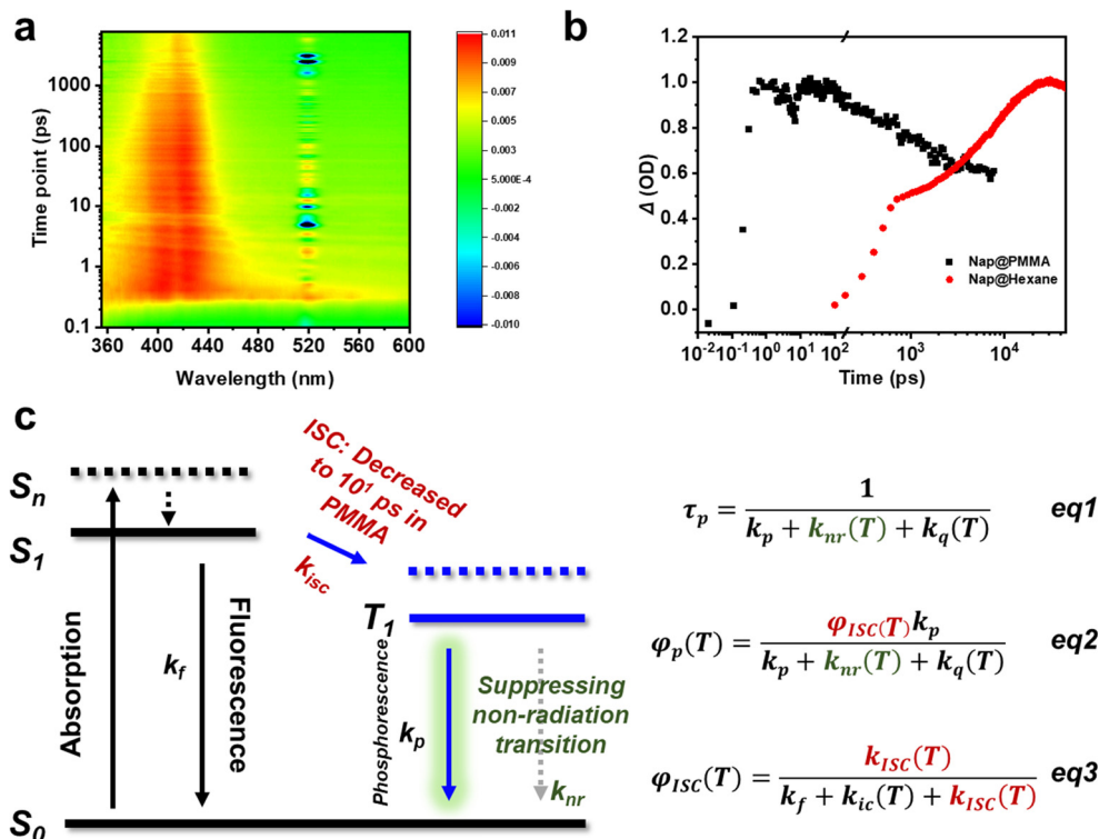
Fig. 3 (a) Transient absorption two-dimensional temporal evolution spectra at room temperature of Nap@PMMA; (b) transient absorption traces of Nap@PMMA at 421 nm and naphthalene in hexane at 421 nm; (c) schematic illustration of a Jablonski diagram for long-lived RTP of the phosphor in our system.
