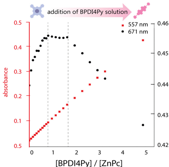
Fig. 2 Plot of the maximum absorbance peaks of ZnPc (671 nm) and BPDIA4Py (557 nm) against the ratio of BPDIA4Py/ZnPc added.
