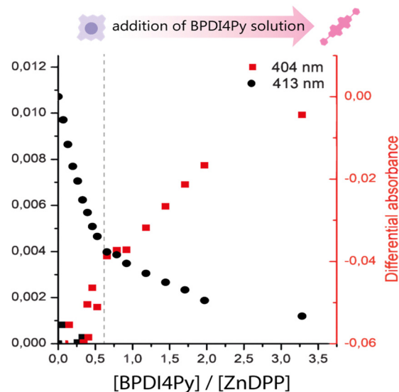
Fig. 3 Plot of the subtracted absorbance peaks of BPDIA4Py (404 nm) and ZnDPP (413 nm) against the ratio of BPDIA4Py/ZnDPP added.
